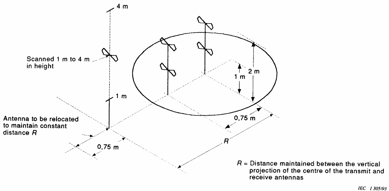
Figure A.2b – Typical antenna positions for alternate site NSA measurements in horizontal polarization for a volume not to exceed 1 m depth, 1,5 m width and 1,5 m height and rear boundary of the volume greater than 1 m from the closest material that may cause undesirable reflections
