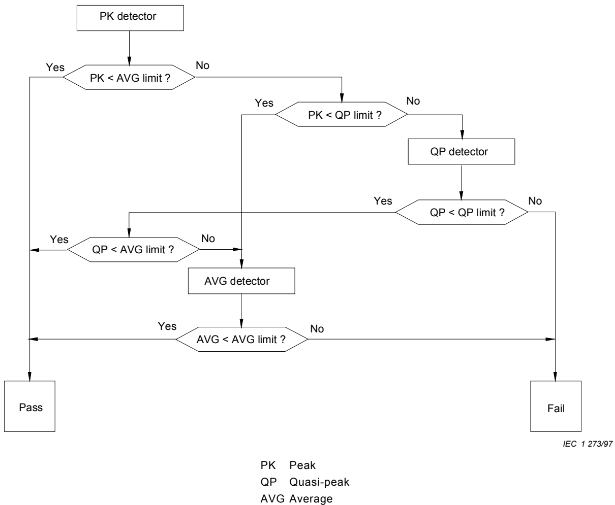
Figure B.1 – Decision tree for peak detector measurements
